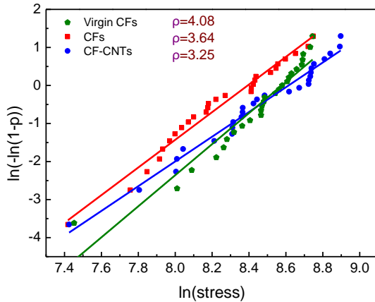
Fig. 5. Weibull plots of tensile treatments.
