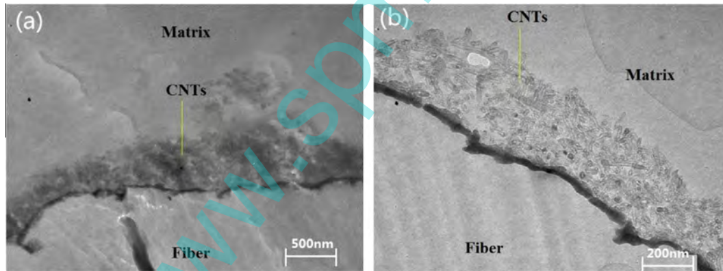
Fig. 14. TEM images of ultrathin section for deposited fiber.
