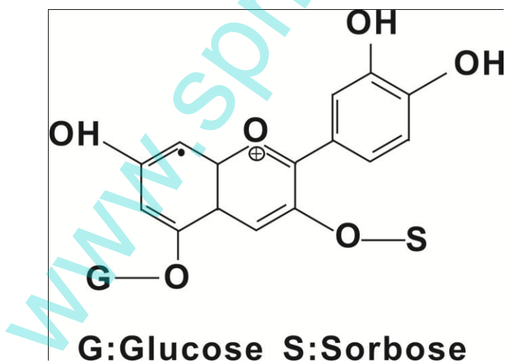
Figure 1. Red cabbage extract of anthocyanin derivatives.
