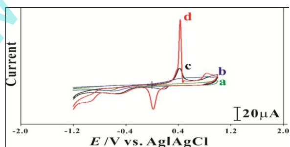
Figure 4. Cyclic voltammograms of (a) 0 % and (b) 5 % of leaf extract in the presence pH 7.0 PBS, The 5 % leaf extract in pH 7.0 PBS containing (c) 0.1 mM and (d) 1mM AgNO_3 . The corresponding CVs have been obtained at 100 \text{ mV s}^{-1} scan rate in the potential range of -1.2 to 1.0 V.
