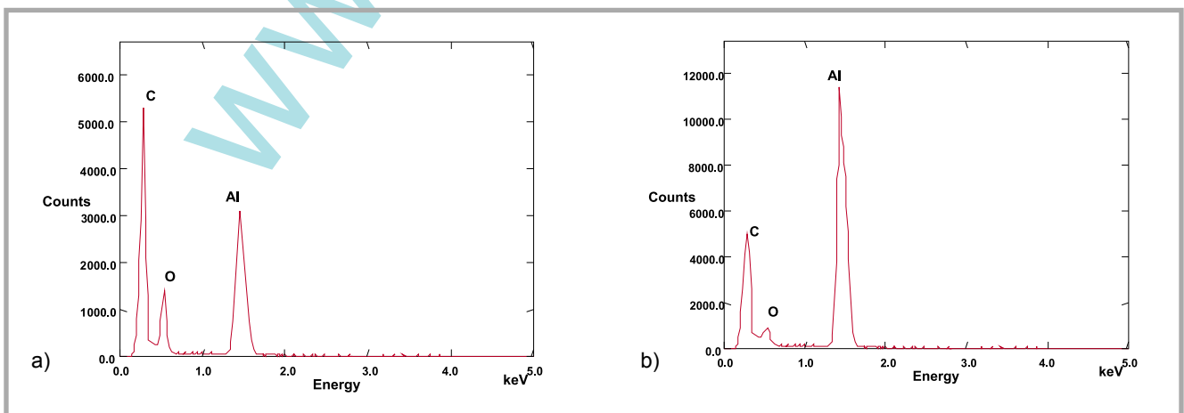
Figure 5. EDX spectra of sputter coated nonwovens: (a) 20 min; (b) 80 min.
