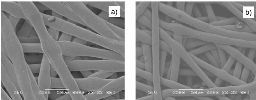
Figure 3. Sputter coated nonwovens observed in SEM: (a) 20 min; (b) 80 min.
